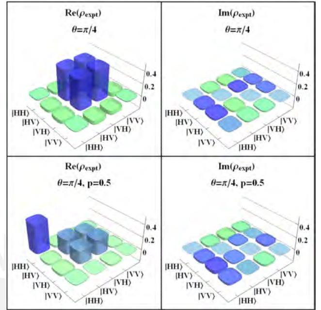
FIG. 2. Real and imaginary parts of the density matrix of a pure state |\psi_{AB}^+\rangle (upper panels) and a mixed, X-type state (lower panels). The measured purity of |\psi_{AB}^+\rangle was 91%, and its fidelity was 0.950 \pm 0.001 . The fidelity of the X state was 0.904 \pm 0.035 .
