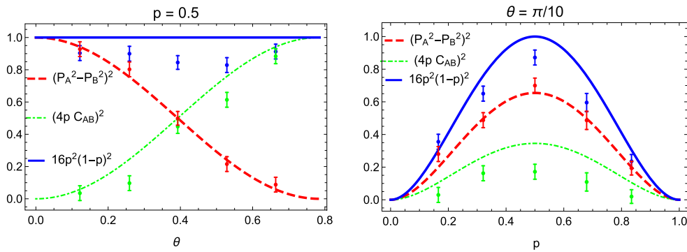
FIG. 4. Experimental test of the constraint given by Eq. (27) in the text. Left: Parameter p is held fixed, and \theta , which characterizes the initial state, varies as shown in the figure. Right: Parameter \theta is held fixed, and parameter p varies as shown in the figure.
