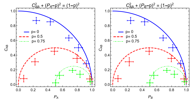
FIG. 3. Experimental tests of the constraints given on top of the graphs. The initial pure state is |\psi_{AB}^+\rangle = \cos \theta |H_A, V_B\rangle + \sin \theta |V_A, H_B\rangle . For p = 0 (state remains pure), curves were parametrized with \theta taking the values \theta = 7.00^\circ, 14.75^\circ, 22.50^\circ, 30.25^\circ, \text{ and } 38.00^\circ . For p = 0.5 and p = 0.75 , the values were \theta = 10.00^\circ, 27.50^\circ, 45.00^\circ, 62.50^\circ, \text{ and } 80.00^\circ .
