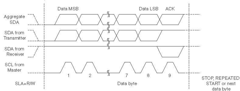
Figure 22-5. Data packet format.
