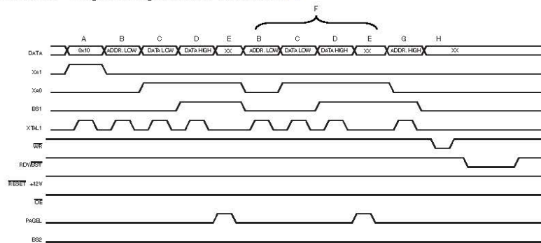
Figure 28-3. Programming the flash waveforms (1) .
