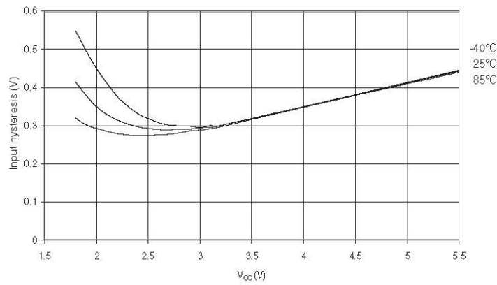
Figure 30-30. I/O pin input hysteresis vs. V_{CC} .
