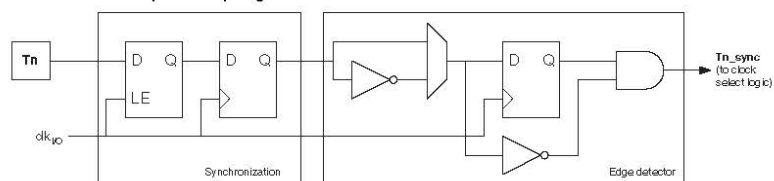
Figure 17-1. T1/T0 pin sampling.
