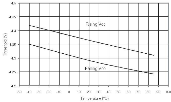
Figure 30-34. BOD thresholds vs. temperature (BODLEVEL is 4.3V).
