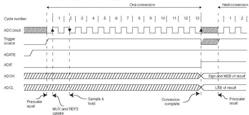
Figure 24-6. ADC timing diagram, auto triggered conversion.
