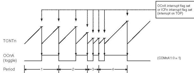
Figure 16-6. CTC mode, timing diagram.
