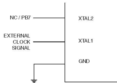
Figure 9-4. External clock drive configuration.
