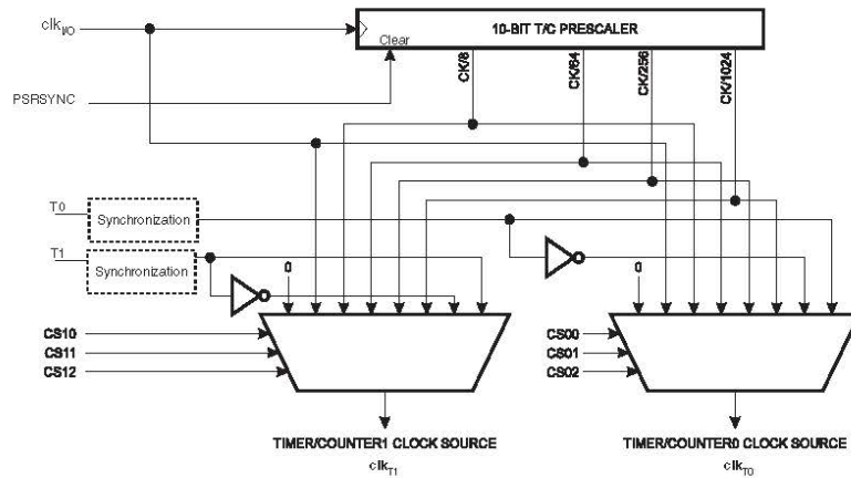
Figure 17-2. Prescaler for timer/counter0 and timer/counter1 (1) .
