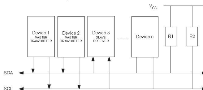
Figure 22-20. An arbitration example.
