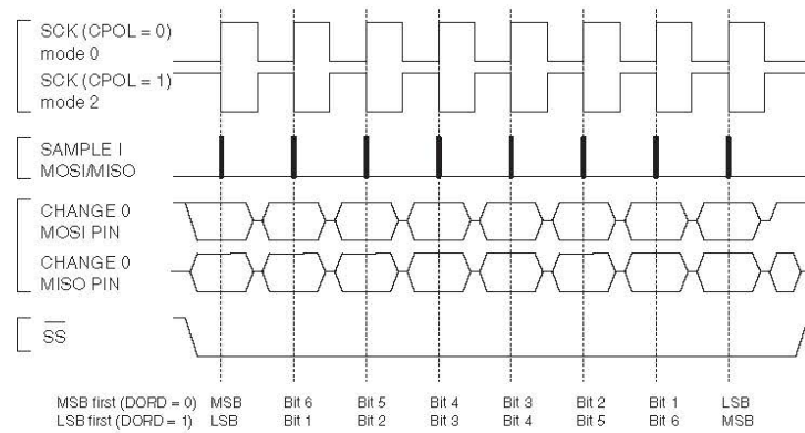
Figure 19-3. SPI transfer format with CPHA = 0.
