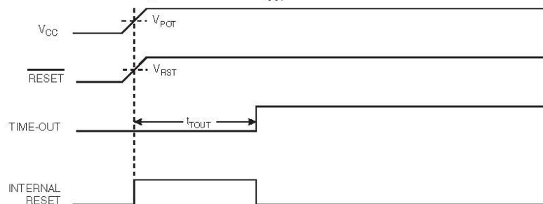
Figure 11-2. MCU start-up, RESETE tied to V_{CC} .
