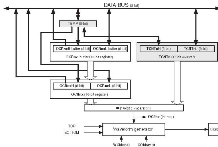
Figure 16-4. Output compare unit, block diagram.
