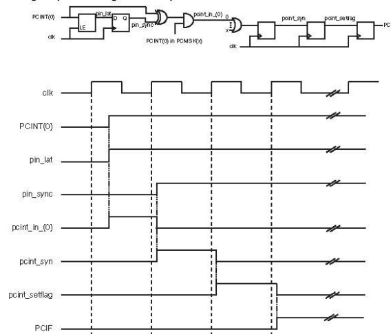
Figure 13-1. Timing of pin change interrupts.
