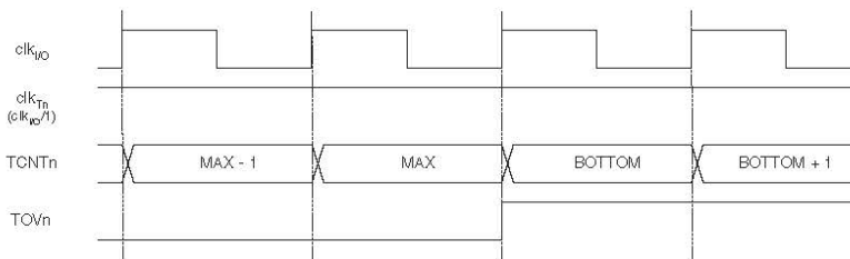
Figure 15-8. Timer/counter timing diagram, no prescaling.
