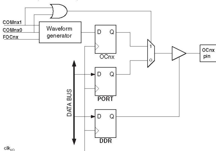
Figure 16-5. Compare match output unit, schematic.
