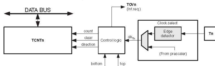
Figure 15-2. Counter unit block diagram.
