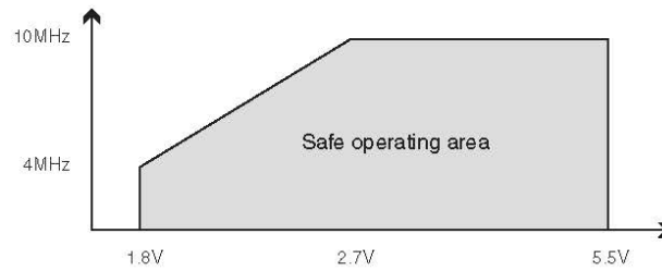
Figure 29-2. Maximum frequency vs. V_{CC} , ATmega48/88/168.
