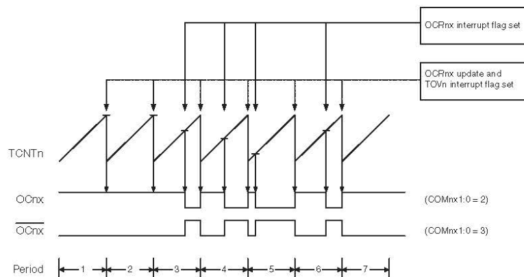
Figure 18-6. Fast PWM mode, timing diagram.
