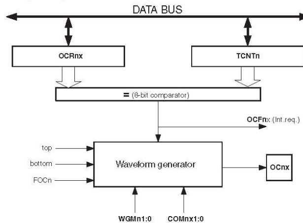
Figure 15-3. Output compare unit, block diagram.
