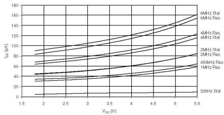
Figure 30-16. Standby supply current vs. V_{CC} (low power crystal oscillator).
