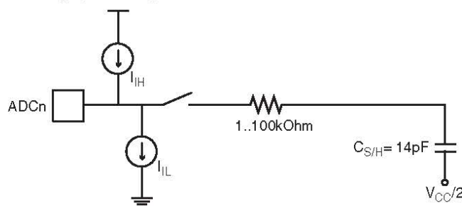
Figure 24-8. Analog input circuitry.
