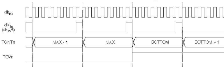
Figure 15-9. Timer/counter timing diagram, with prescaler ( f_{clk_{I/O}}/8 ).
