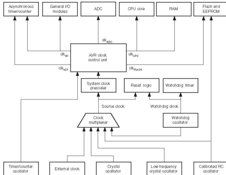
Figure 9-1. Clock distribution.
