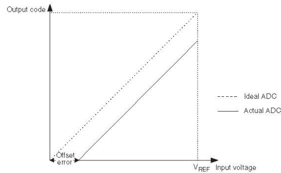
Figure 24-10. Offset error.
