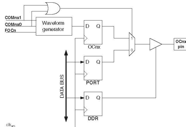
Figure 15-4. Compare match output unit, schematic.
