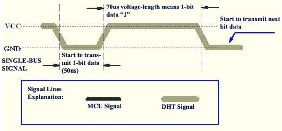
Figure 5 Data "1" Indication
