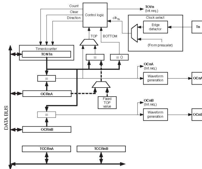
Figure 18-1. 8-bit timer/counter block diagram.
