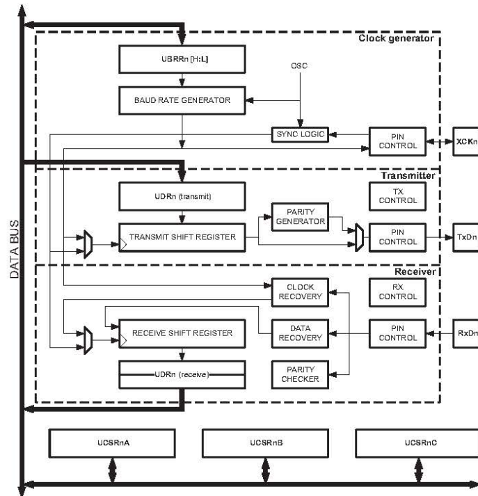
Figure 20-1. USART block diagram (1) .
