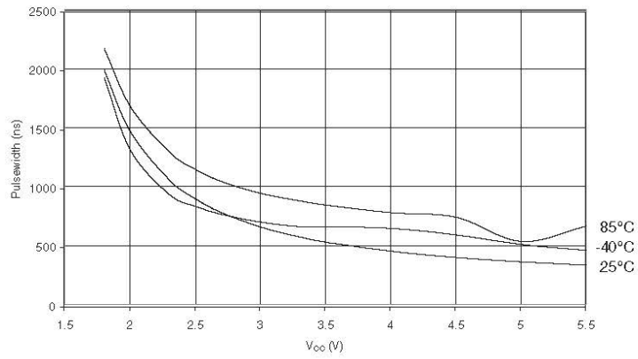
Figure 30-51. Reset pulse width vs. V_{CC} .
