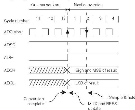
Figure 24-7. ADC timing diagram, free running conversion.
