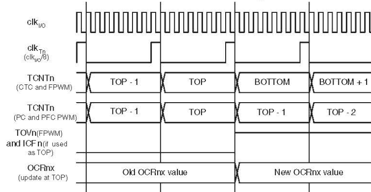
Figure 16-13. Timer/counter timing diagram, with prescaler ( f_{clk_{IO}}/8 ).
