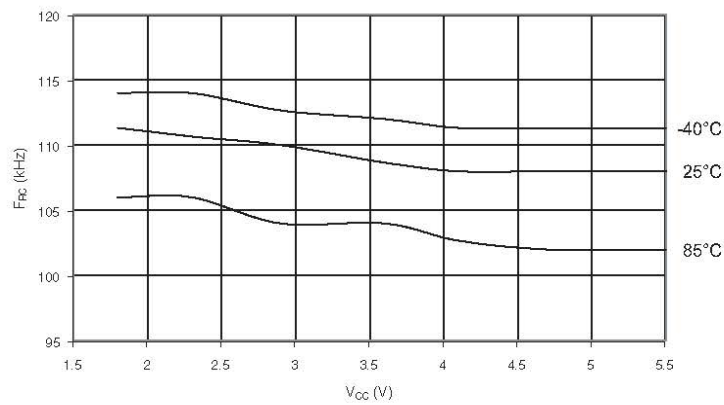
Figure 30-40. Watchdog oscillator frequency vs. V_{CC} .
