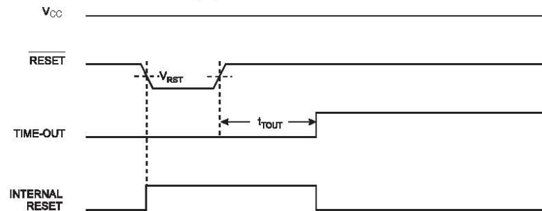
Figure 11-4. External reset during operation.
