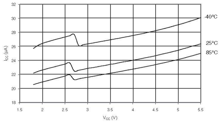
Figure 30-44. Brownout detector current vs. V_{CC} .
