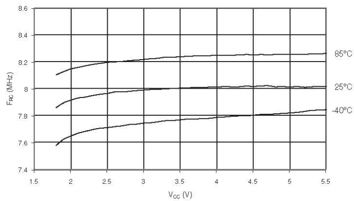
Figure 30-42. Calibrated 8MHz RC oscillator frequency vs. V CC .
