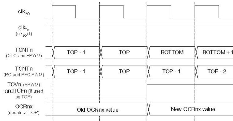
Figure 16-12. Timer/counter timing diagram, no prescaling.
