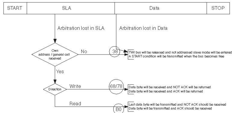
Figure 22-21. Possible status codes caused by arbitration.
