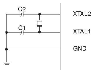
Figure 9-2. Crystal oscillator connections.
