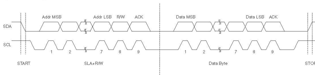
Figure 22-6. Typical data transmission.
