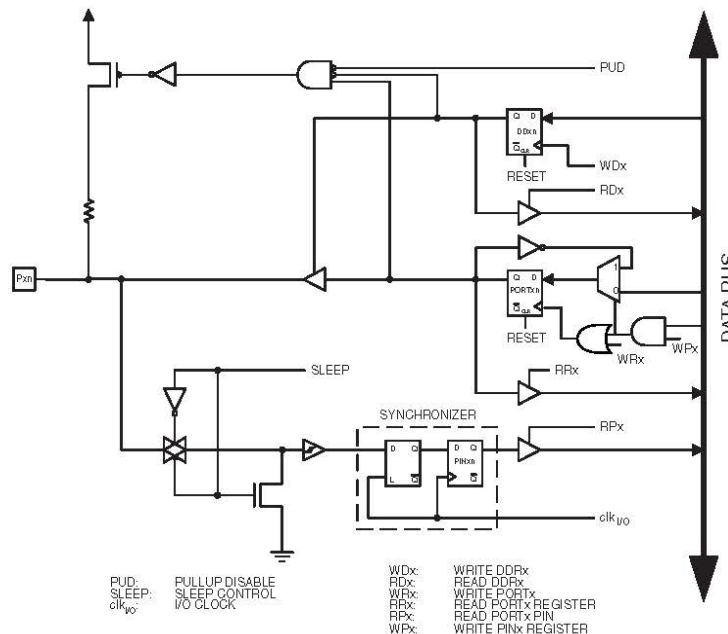
Figure 14-2. General digital I/O (1) .
