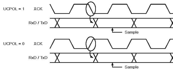
Figure 20-3. Synchronous mode XCKn timing.
