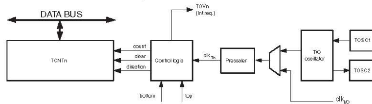
Figure 18-2. Counter unit block diagram.
