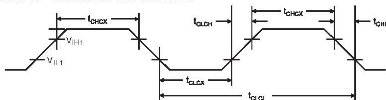
Figure 29-3. External clock drive waveforms.
