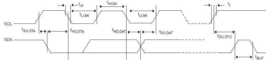
Figure 29-4. 2-wire serial bus timing.
