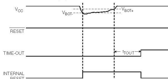
Figure 11-5. Brown-out reset during operation.
