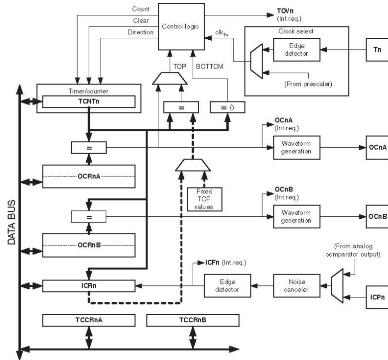
Figure 16-1. 16-bit timer/counter block diagram (1) .
