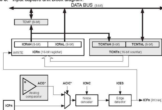
Figure 16-3. Input capture unit block diagram.
