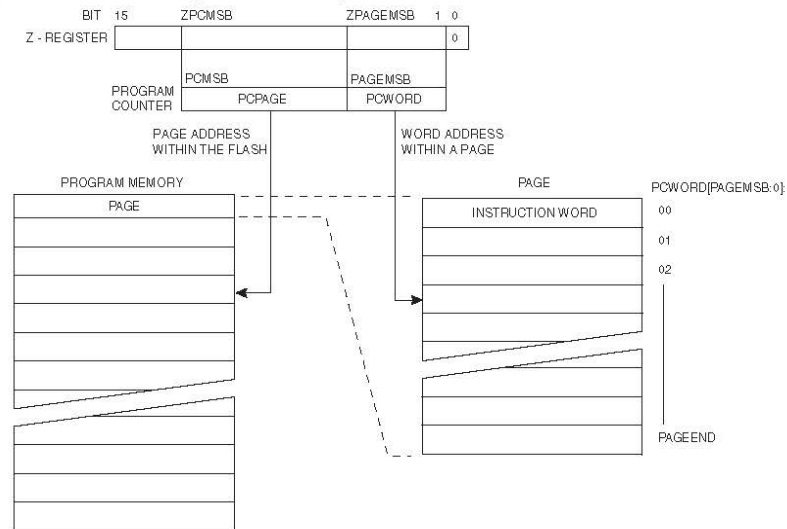
Figure 27-3. Addressing the flash during SPM (1) .
