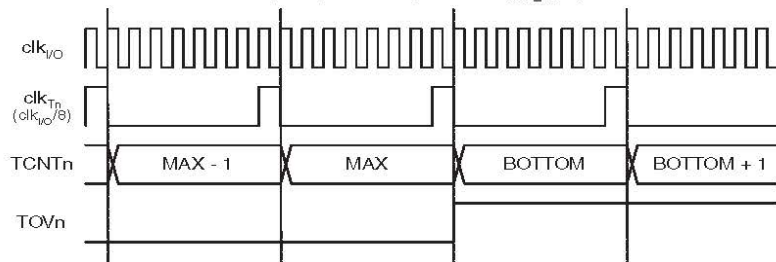
Figure 18-9. Timer/counter timing diagram, with prescaler ( f_{clk_{I/O}}/8 ).
