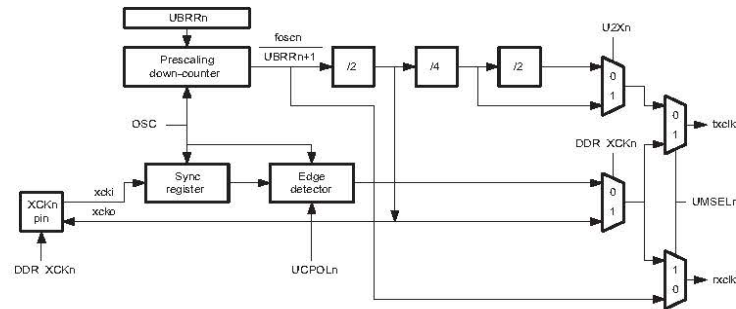
Figure 20-2. Clock generation logic, block diagram.
