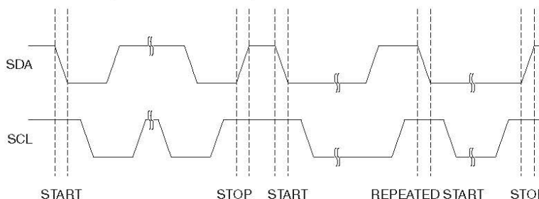
Figure 22-3. START, REPEATED START, and STOP conditions.
