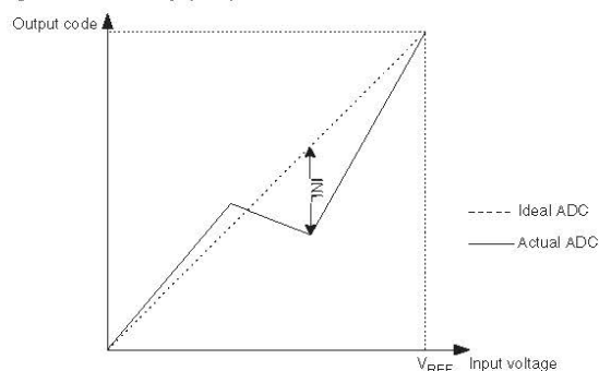
Figure 24-12. Integral non-linearity (INL).
