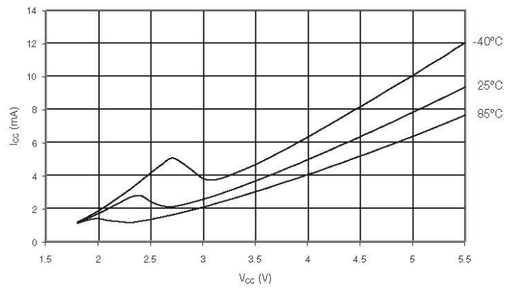
Figure 30-48. Programming current vs. V_{CC} .
