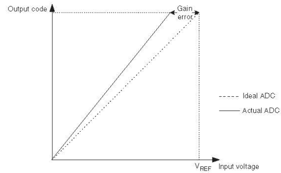
Figure 24-11. Gain error.
