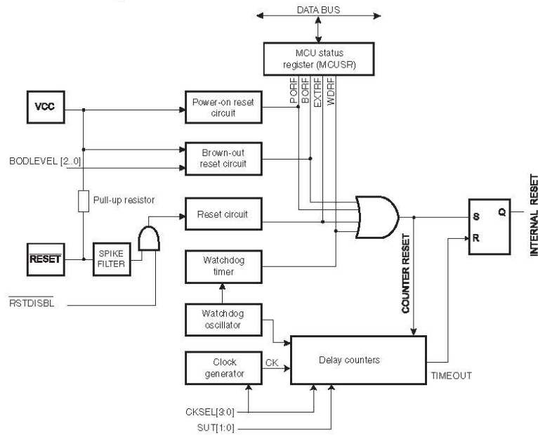
Figure 11-1. Reset logic.
