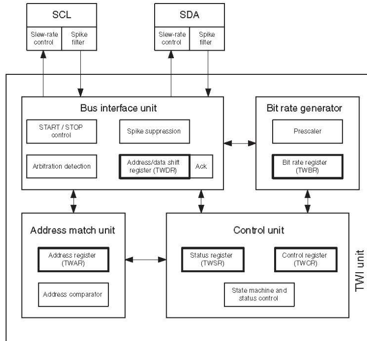
Figure 22-9. Overview of the TWI module.
