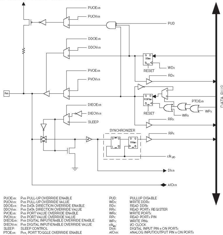
Figure 14-5. Alternate port functions (1) .
