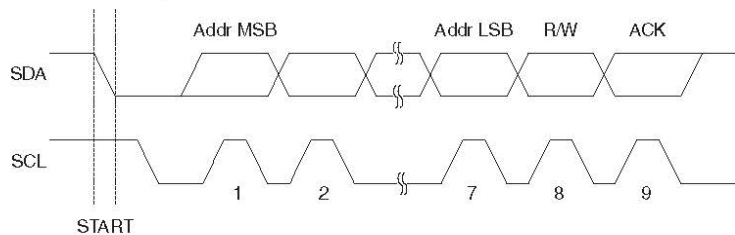
Figure 22-4. Address packet format.
