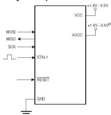
Figure 28-7. Serial programming and verify (1) .
