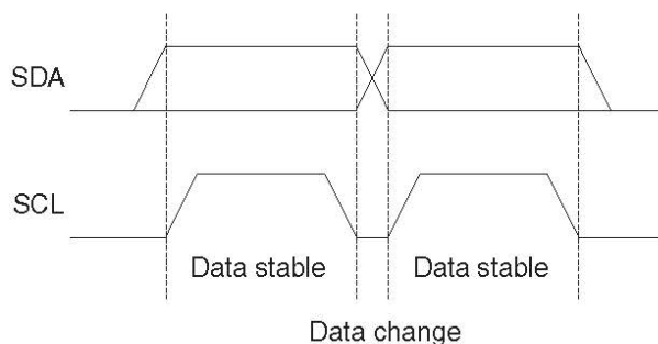
Figure 22-2. Data validity.
