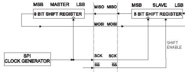
Figure 19-2. SPI master-slave interconnection.
