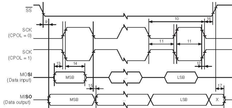
Figure 29-6. SPI interface timing requirements (slave mode).
