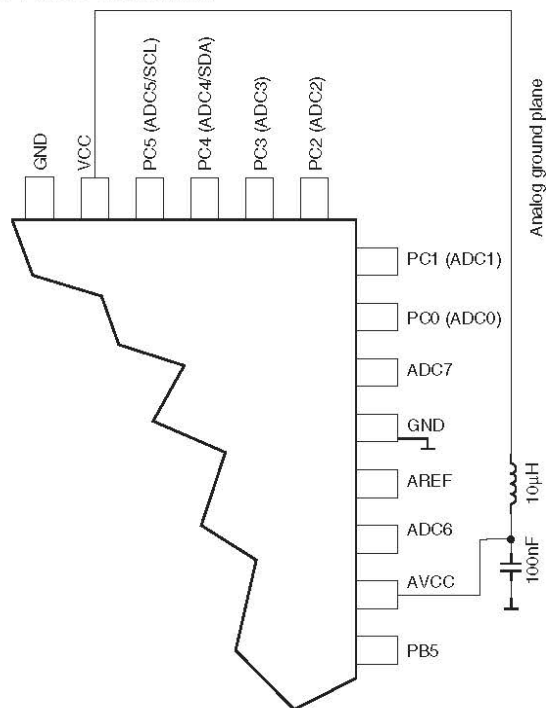
Figure 24-9. ADC power connections.
