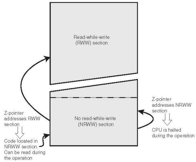
Figure 27-1. Read-while-write vs. no read-while-write.
