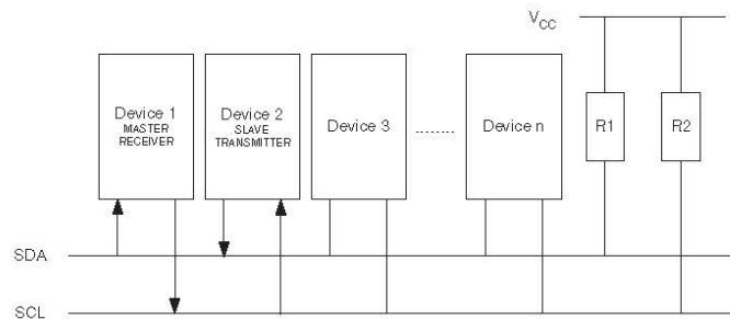
Figure 22-13. Data transfer in master receiver mode.
