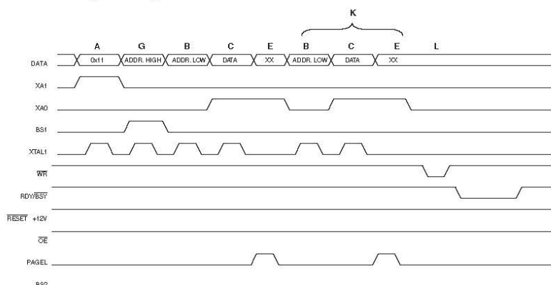
Figure 28-4. Programming the EEPROM waveforms.
