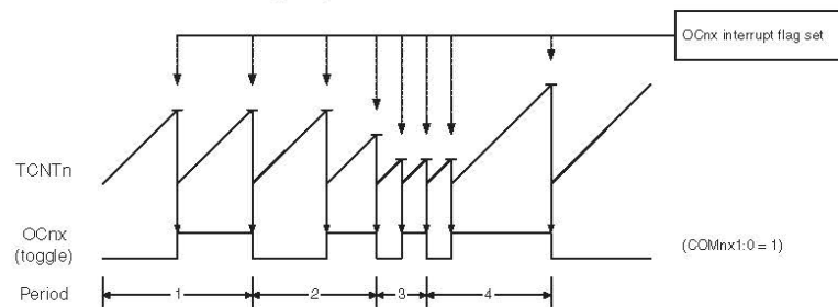
Figure 18-5. CTC mode, timing diagram.
