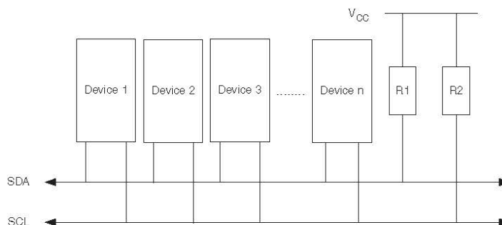
Figure 22-1. TWI bus interconnection.
