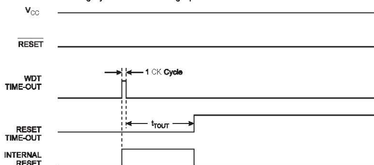
Figure 11-6. Watchdog system reset during operation.
