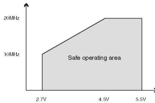
Figure 29-2. Maximum frequency vs. V_{CC} , ATmega48/88/168.
