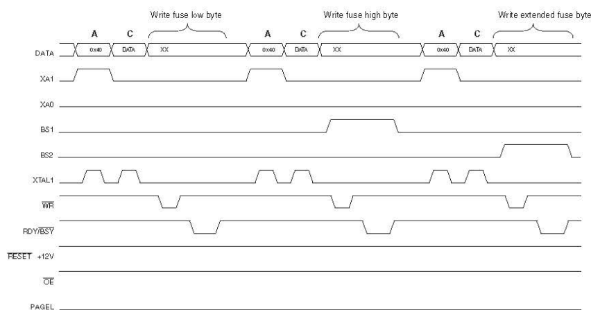
Figure 28-5. Programming the FUSES waveforms.
