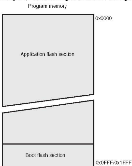
Figure 8-2. Program memory map, Atmel ATmega88 and Atmel ATmega168.
