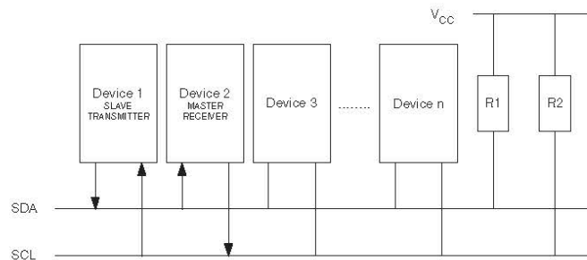
Figure 22-17. Data transfer in slave transmitter mode.
