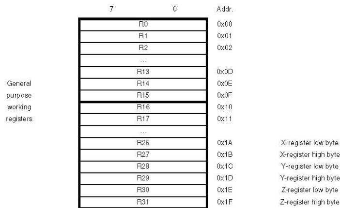
Figure 7-2. AVR CPU general purpose working registers.
