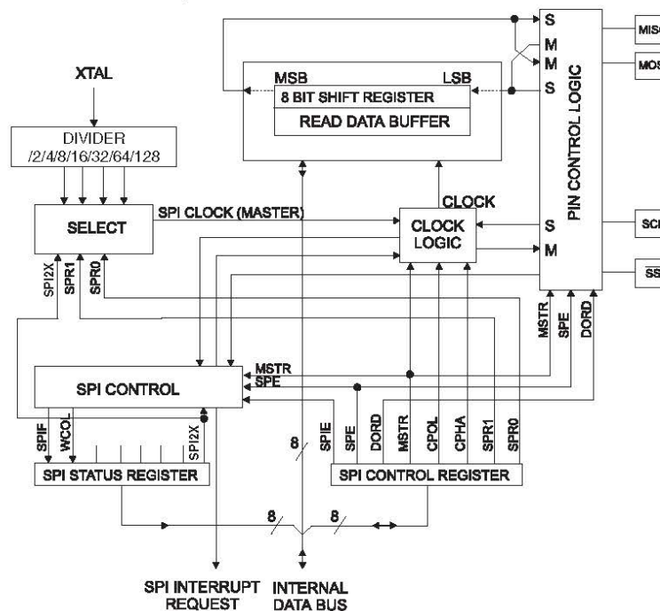
Figure 19-1. SPI block diagram (1) .
