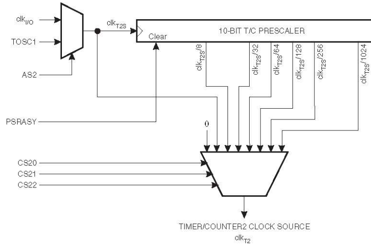
Figure 18-12. Prescaler for Timer/Counter2.
