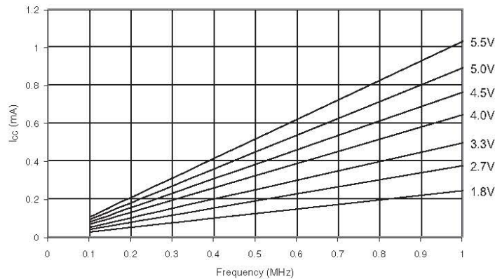
Figure 30-1. Active supply current vs. frequency (0.1MHz - 1.0MHz).
