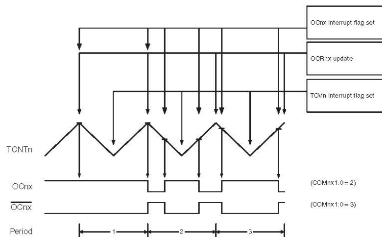
Figure 18-7. Phase correct PWM mode, timing diagram.
