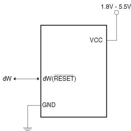
Figure 25-1. The debugWIRE setup.
