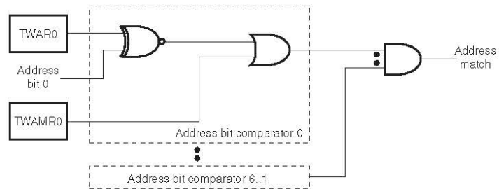
Figure 22-22. TWI address match logic, block diagram.
