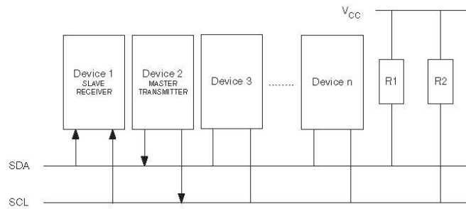
Figure 22-15. Data transfer in slave receiver mode.
