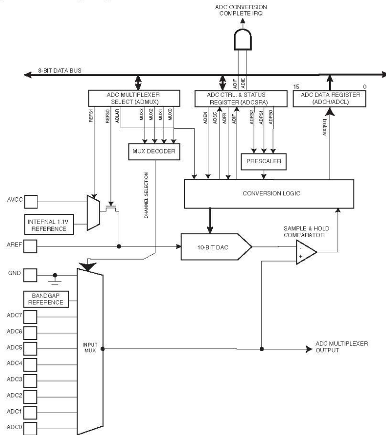
Figure 24-1. Analog to digital converter block schematic operation.
