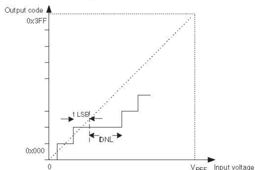
Figure 24-13. Differential non-linearity (DNL).
