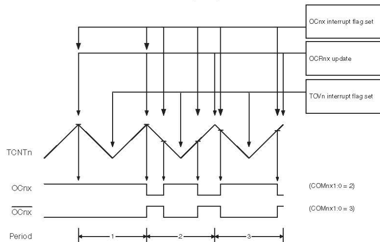
Figure 15-7. Phase correct PWM mode, timing diagram.
