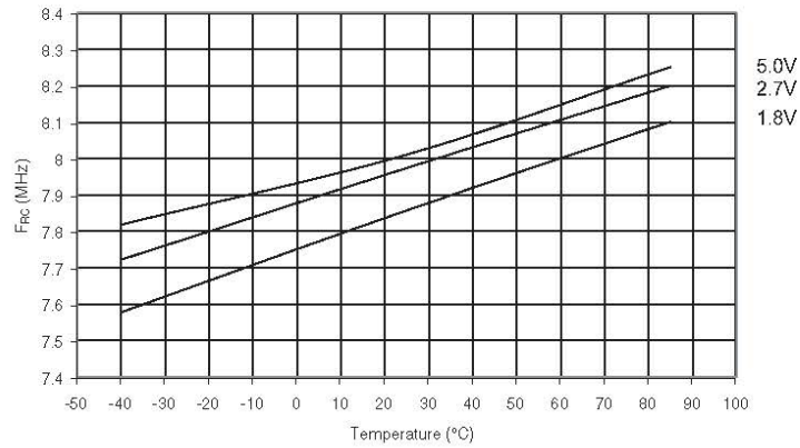
Figure 30-42. Calibrated 8MHz RC oscillator frequency vs. V CC .
