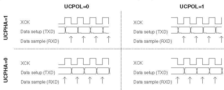
Figure 21-1. UCPHAn and UCPOLn data transfer timing diagrams.
