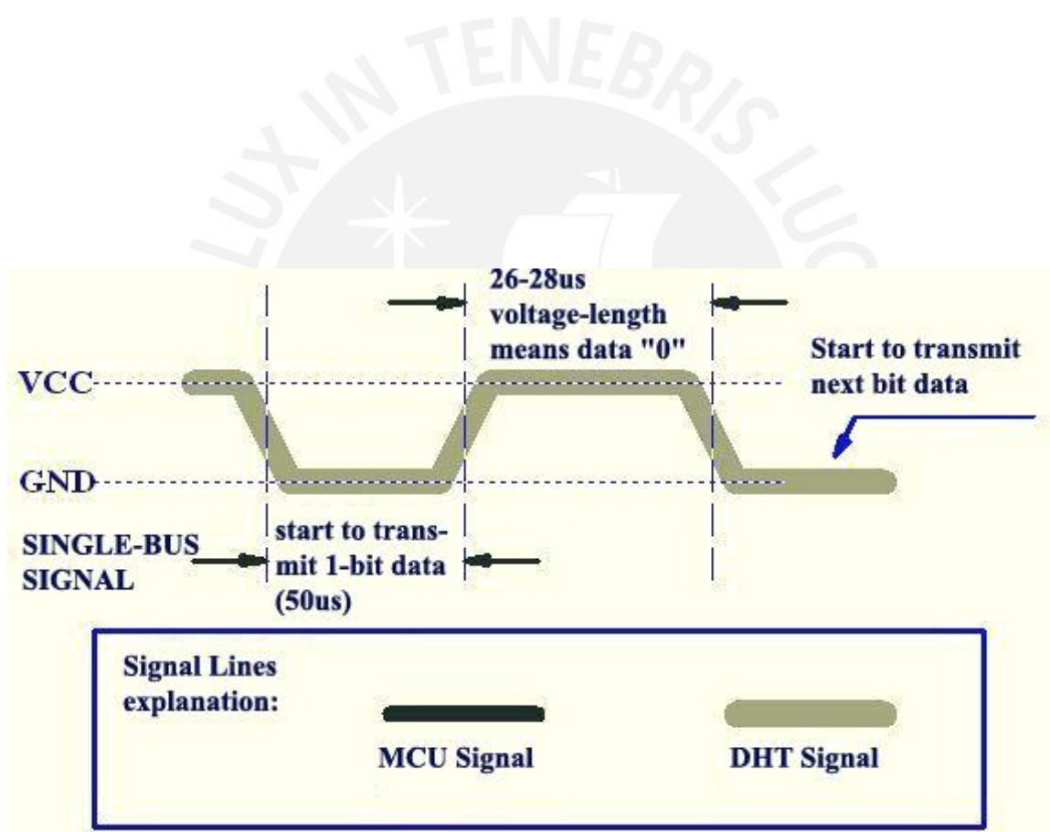
Figure 4 Data "0" Indication
