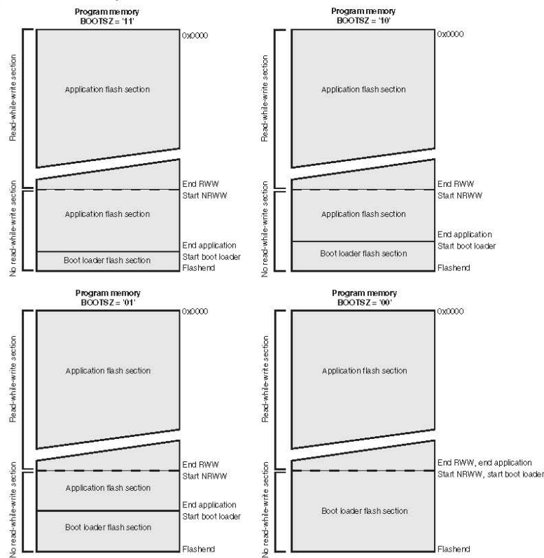
Figure 27-2. Memory sections.
