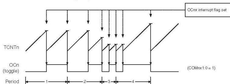
Figure 15-5. CTC mode, timing diagram.
