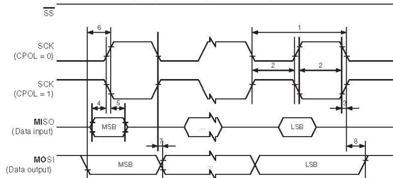
Figure 29-5. SPI interface timing requirements (master mode).
