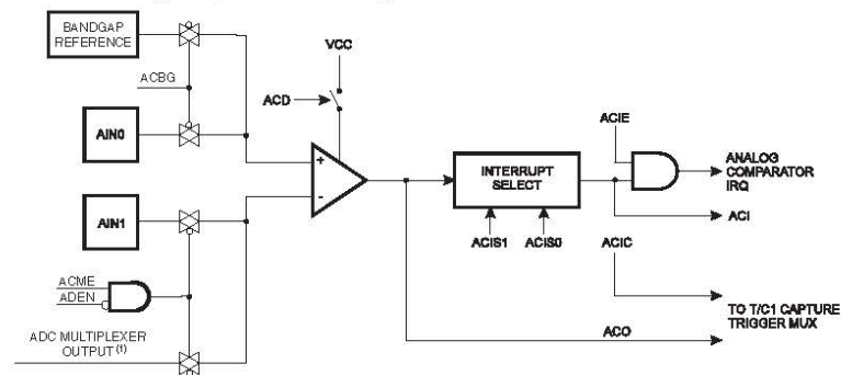
Figure 23-1. Analog comparator block diagram (2) .
