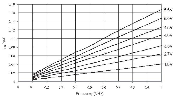
Figure 30-7. Idle supply current vs. frequency (0.1MHz - 1.0MHz).
