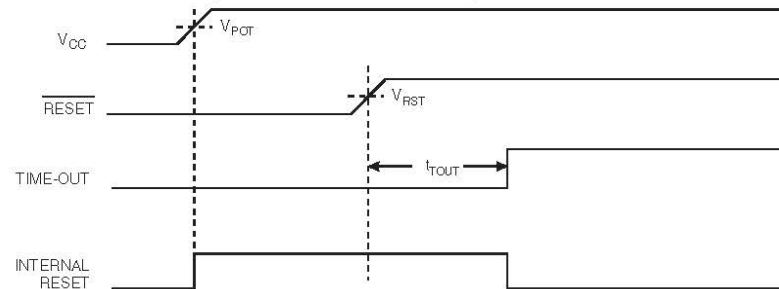
Figure 11-3. MCU start-up, \overline{\text{RESET}} extended externally.
