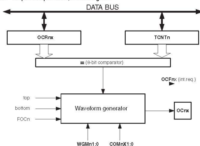
Figure 18-3. Output compare unit, block diagram.
