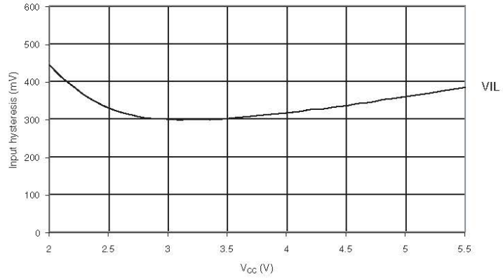
Figure 30-33. Reset input pin hysteresis vs. V_{CC}
