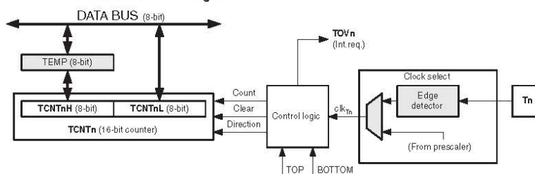
Figure 16-2. Counter unit block diagram.
