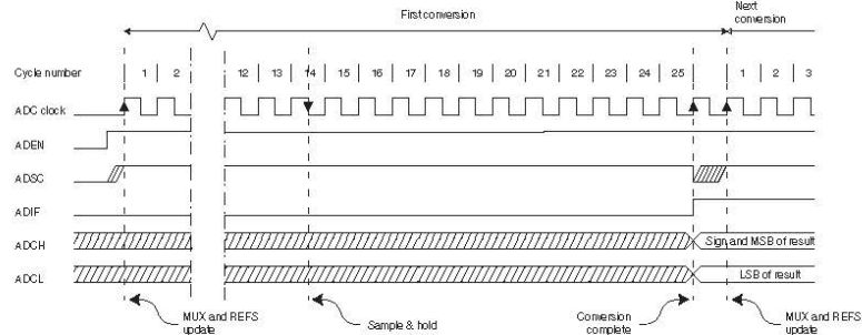
Figure 24-5. ADC timing diagram, single conversion.
