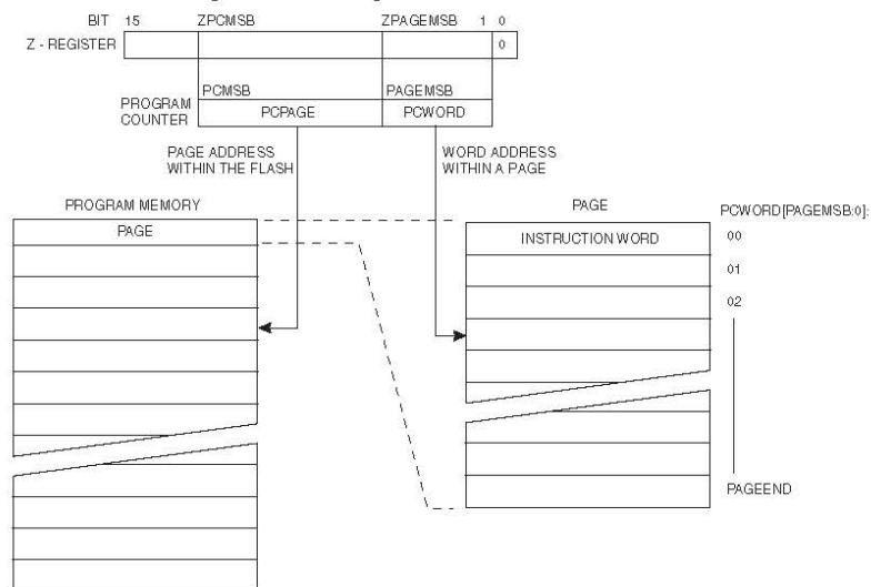
Figure 26-1. Addressing the flash during SPM (1) .
