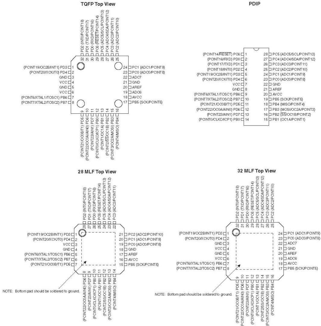
Figure 1-1. Pinout Atmel ATmega48/88/168.
