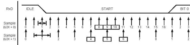
Figure 20-5. Start bit sampling.
