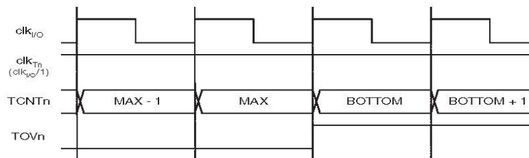
Figure 18-8. Timer/counter timing diagram, no prescaling.
