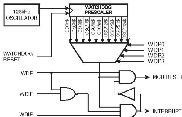
Figure 11-7. Watchdog timer.
