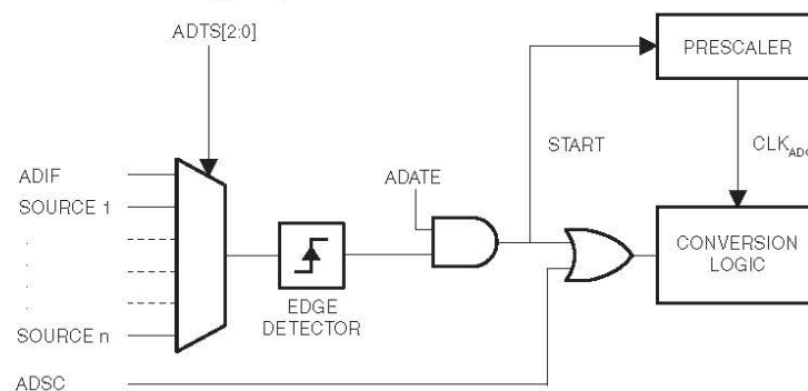
Figure 24-2. ADC auto trigger logic.
