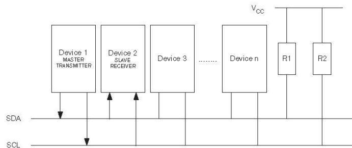
Figure 22-11. Data transfer in master transmitter mode.
