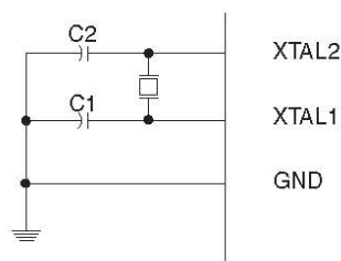
Figure 9-3. Crystal oscillator connections.
