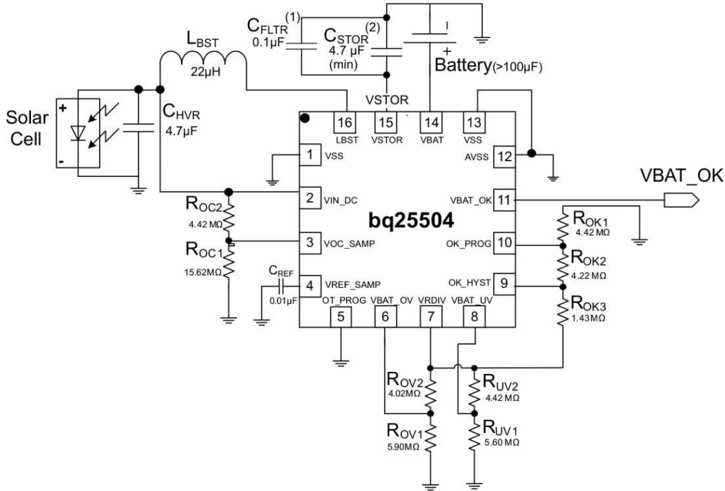
Figure 2. Typical Solar Application Circuit
