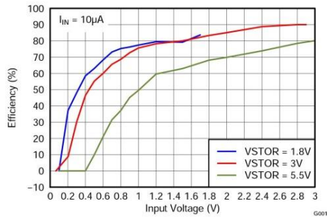
Figure 6. Efficiency vs Input Voltage
