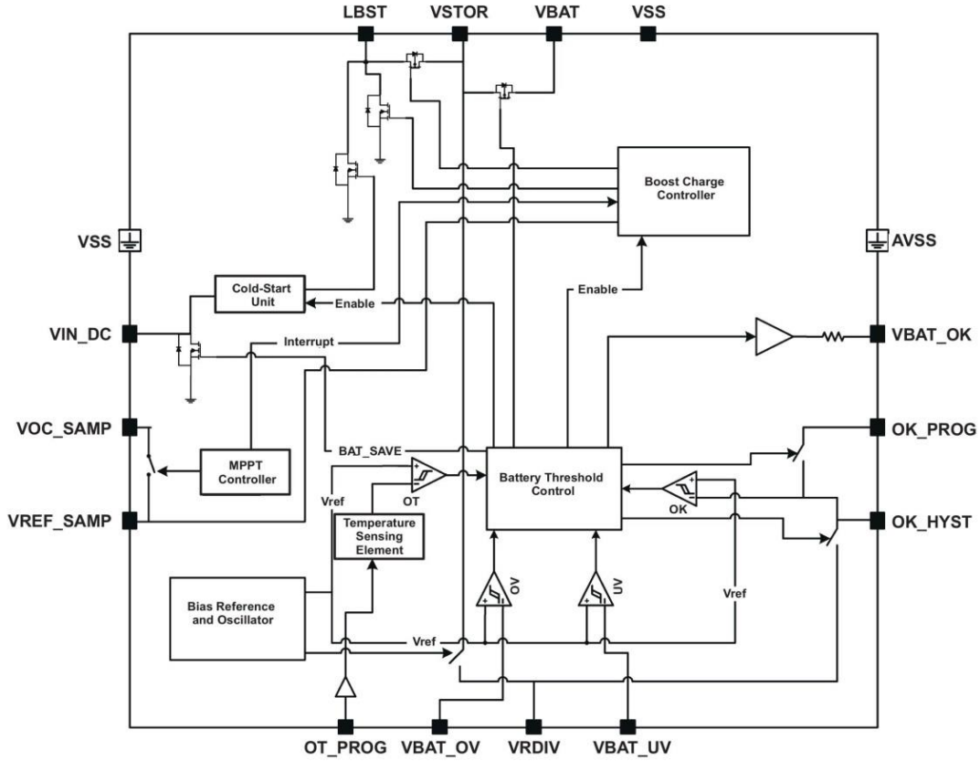
Figure 5. High-level Functional Diagram
