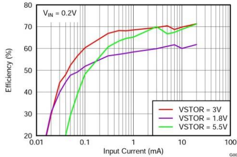
Figure 12. Efficiency vs Input Current
