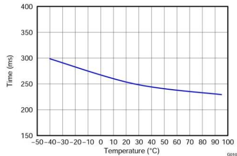
Figure 15. Settling Period vs Temperature
