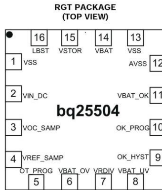
Figure 1. bq25504 3mm x 3mm QFN-16 Package
