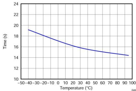
Figure 14. Sample Period vs Temperature
