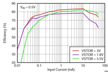
Figure 11. Efficiency vs Input Current
