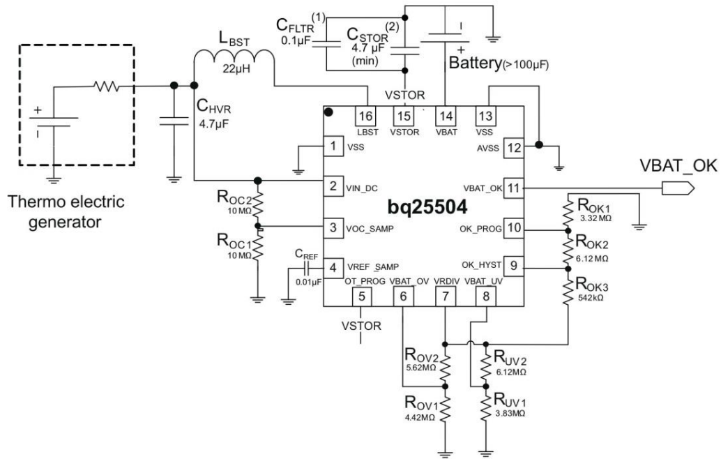
Figure 3. Typical TEG Application Circuit
