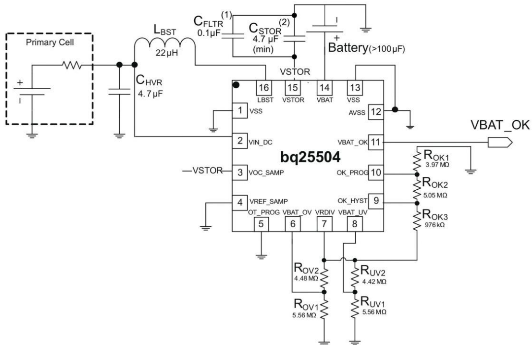
Figure 4. Typical MPPT Disabled Application Circuit
