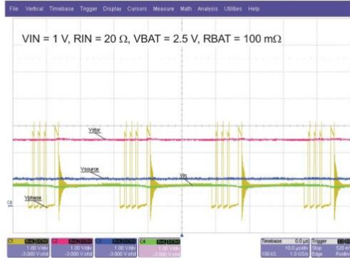
Figure 18. Example of PFM Switching Converter Waveform
