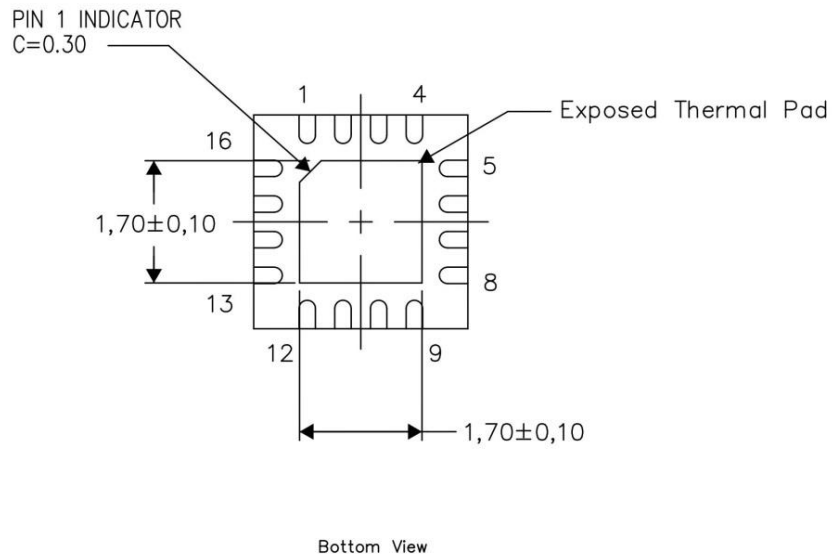
Exposed Thermal Pad Dimensions
