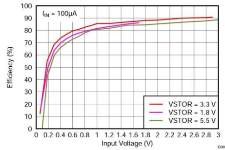
Figure 7. Efficiency vs Input Voltage
