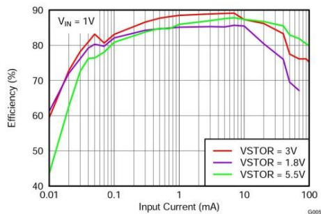
Figure 10. Efficiency vs Input Current
