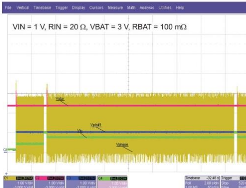
Figure 21. Example of Sampling Time for MPPT Operation
