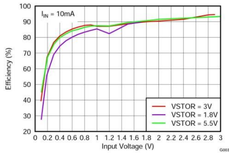
Figure 8. Efficiency vs Input Voltage
