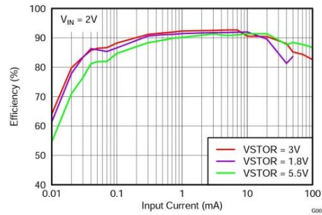
Figure 9. Efficiency vs Input Current
