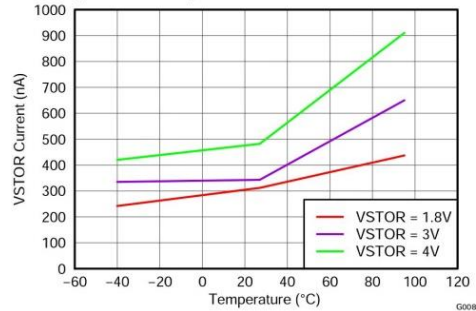
Figure 13. VSTOR Quiescent Current vs Temperature
