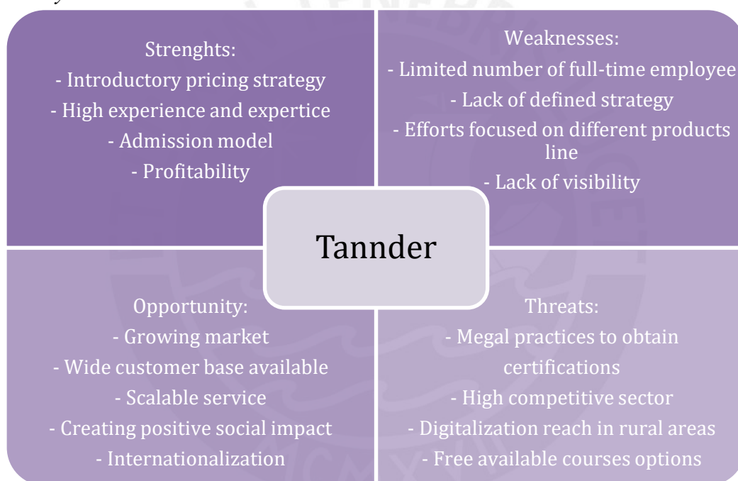
Figure 4 SWOT analysis
